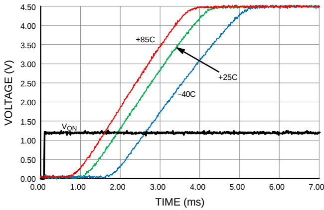
Figure 25. Turn-On Response ( V_{IN} = 4.5\text{ V} , C_{IN} = 10\mu F , C_L = 1\mu F , R_L = 50\Omega )
