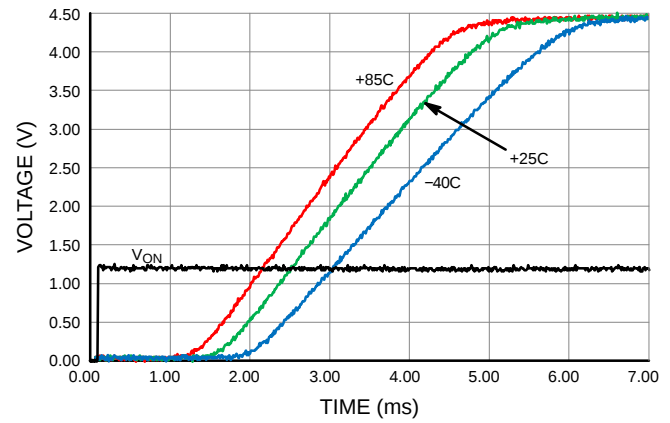
Figure 26. Turn-On Response ( V_{IN} = 4.5\text{ V} , C_{IN} = 10\mu F , C_L = 100\mu F , R_L = 5\Omega )
