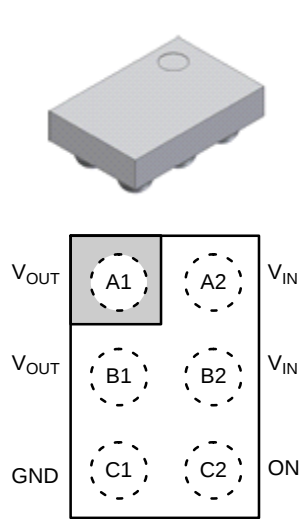
Figure 3. Top View
