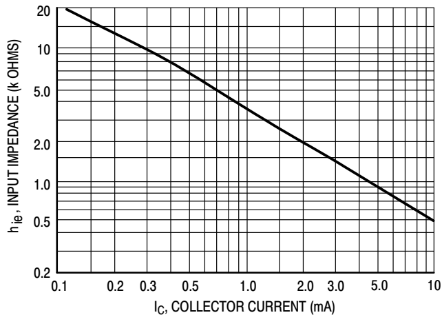
Figure 13. Input Impedance
