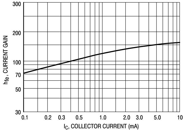
Figure 11. Current Gain
