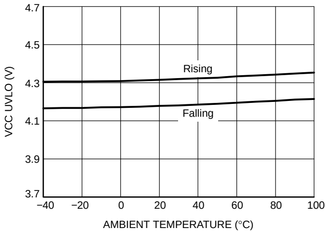
Figure 4. V_{CC}\text{ UVLO} vs. Temperature ( EN = 5\text{ V} )
