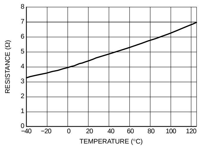
Figure 9. R_{OL}
