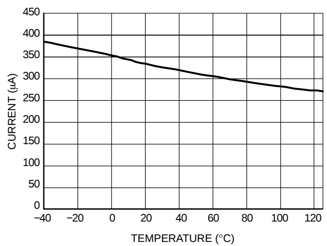
Figure 15. I_{CC4}
