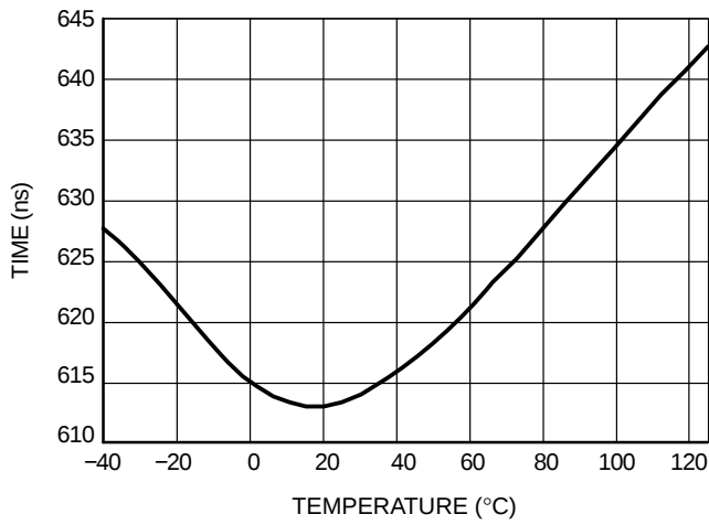
Figure 16. T_{dead} (B Version)
