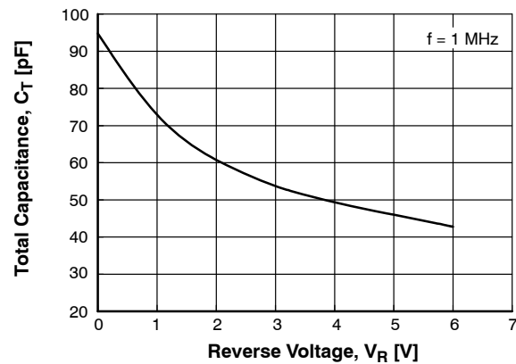
Figure 3. Total Capacitance
