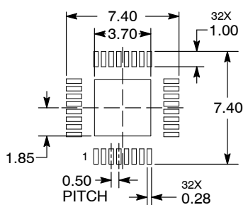
BOTTOM VIEW RECOMMENDED SOLDERING FOOTPRINT*
