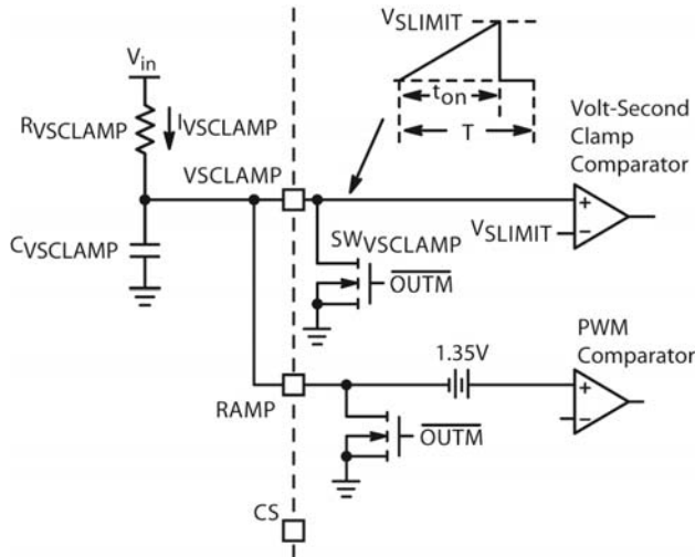
Figure 53. The VSCLAMP Configuration in Voltage-mode Control
