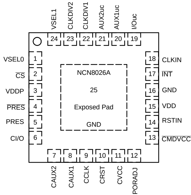
Figure 2. NCN8026A – QFN-24 Pinout (Top View)
