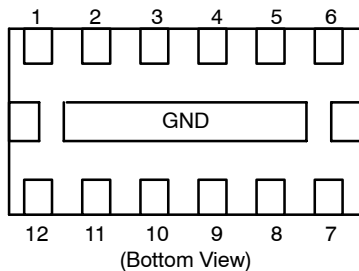
Figure 3. Pin Diagram
