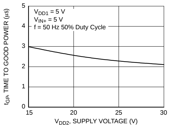
Figure 32. Time to Good Power ( t_{\text{GP}} ) vs. Supply Voltage ( V_{DD2} )
