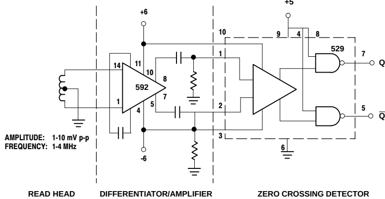
READ HEAD
