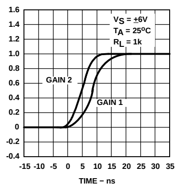
Figure 4. Pulse Response
