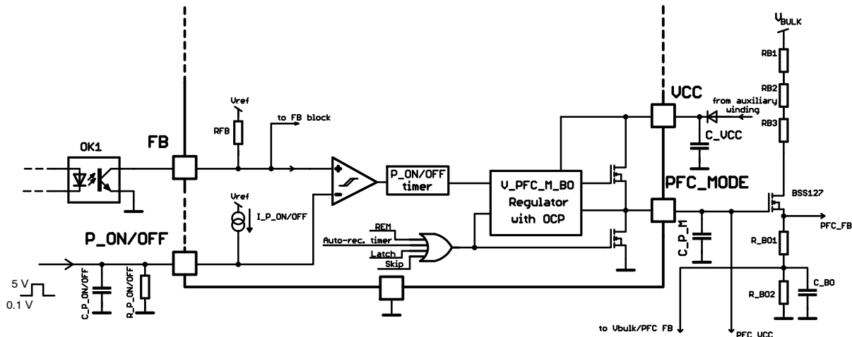
Figure 42. Internal Connection of the PFC MODE and P ON/OFF Blocks
