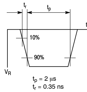
INPUT PULSE
