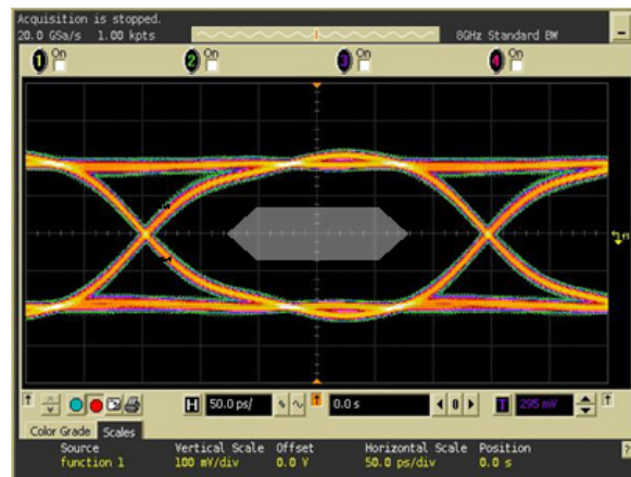
Figure 12. HDMI1.4 Eye Diagram with and without MG2040. 3.4 Gb/s, 400 mV pp
