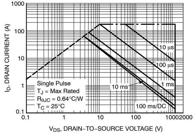
Figure 14. Safe Operating Area
