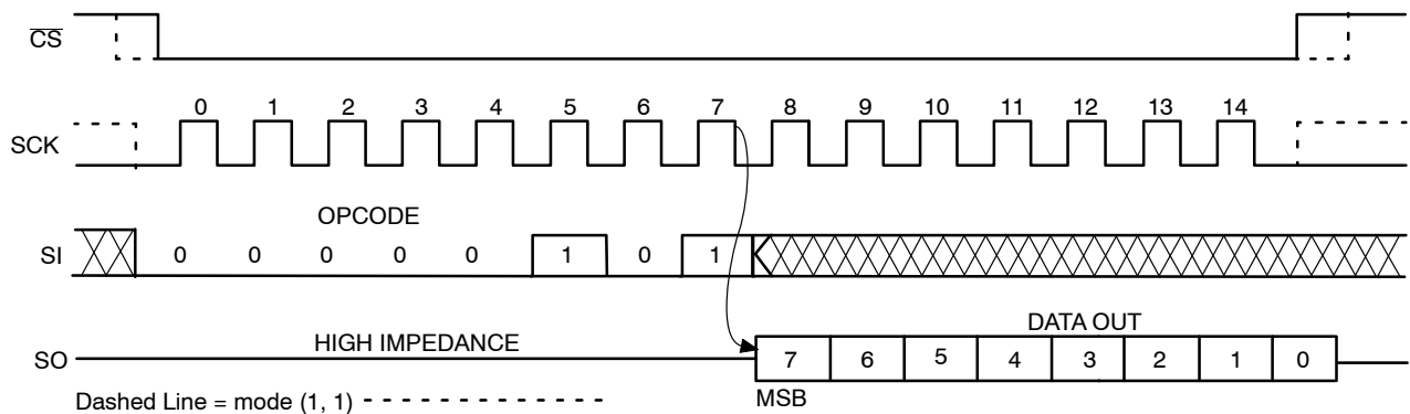
Figure 10. RDSR Timing
