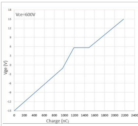
Figure 10. Gate Voltage vs. Gate Charge
