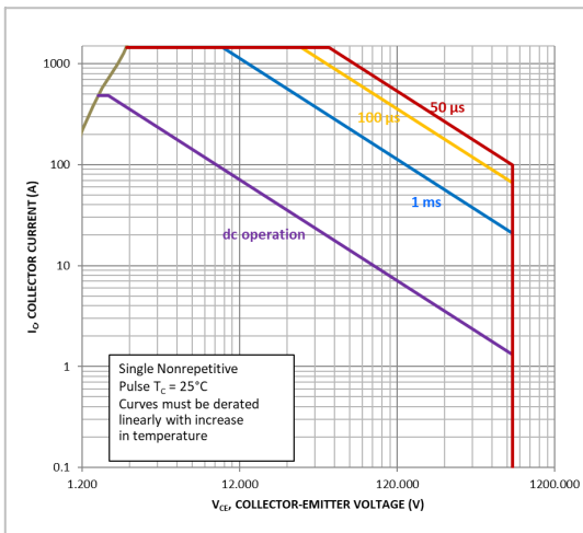
Figure 8. FBSOA (T1, T4)
