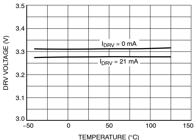
Figure 18. DRV Voltage vs. Junction Temperature
