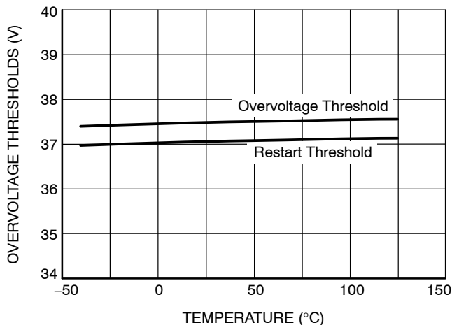
Figure 16. Input Overvoltage Thresholds vs. Junction Temperature
