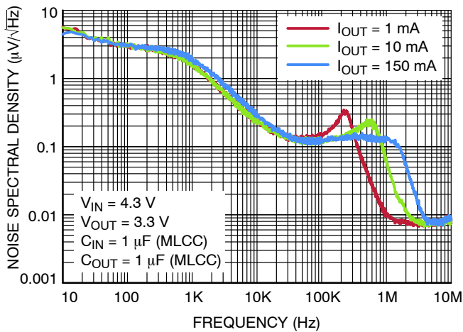
Figure 23. Output Voltage Noise Spectral Density – V_{OUT} = 3.3 V
