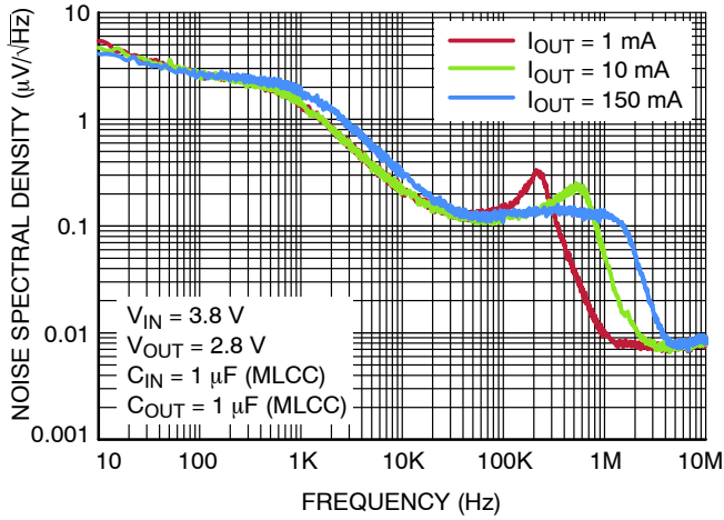
Figure 22. Output Voltage Noise Spectral Density – V_{OUT} = 2.8 V
