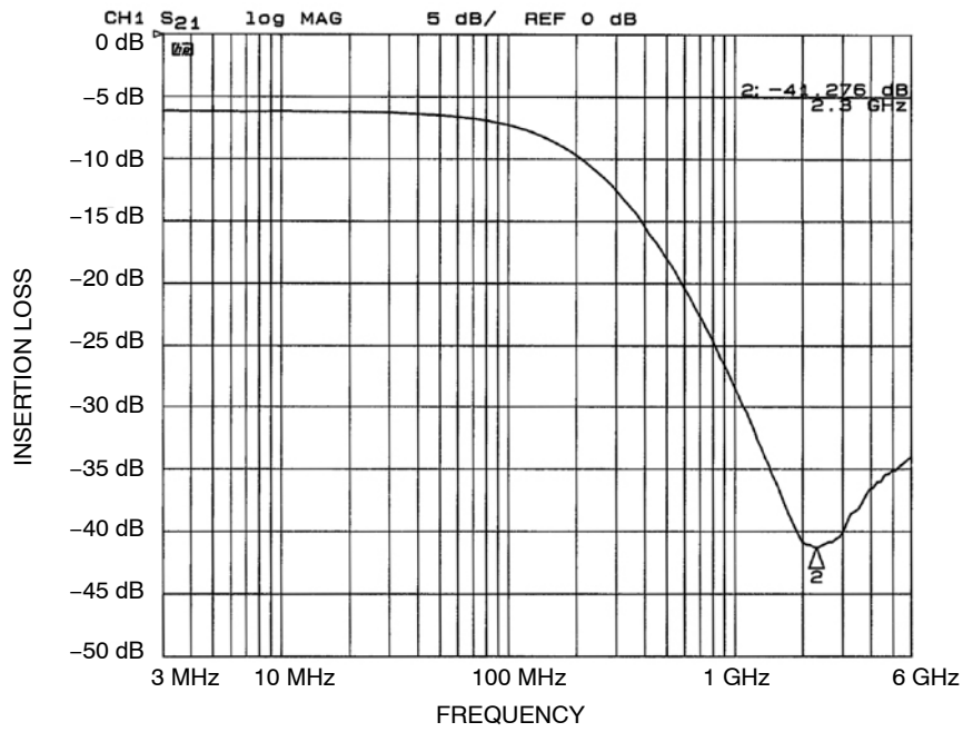
Figure 7. Insertion Loss vs. Frequency (FILTER3 Input to GND, CM1630-06DE)
