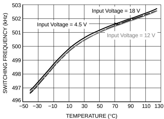
Figure 12. Switching Frequency vs. Temperature
