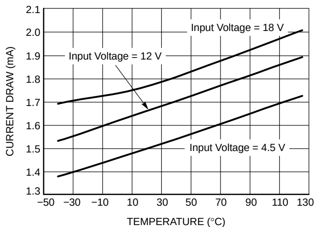
Figure 10. NCP3170 Enabled Current vs. Temperature
