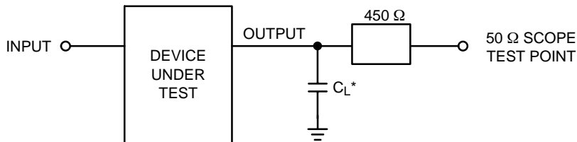
Figure 4. Test Circuit
