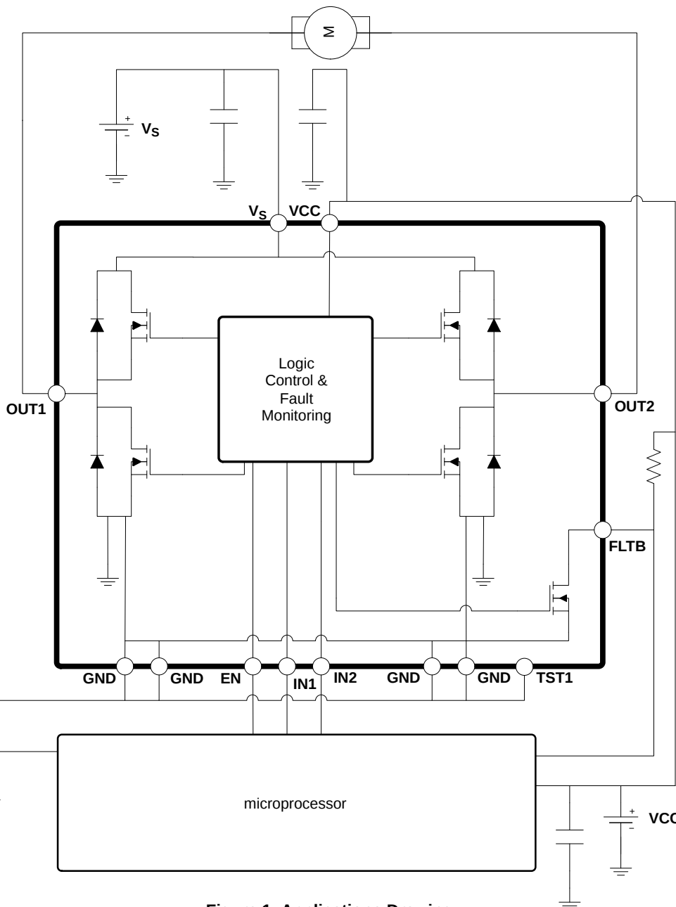
Figure 1. Applications Drawing
