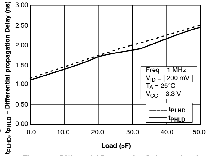
Figure 16. Differential Propagation Delay vs. Load
