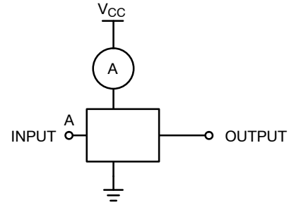
Figure 5. I_{CCD} Test Circuit
