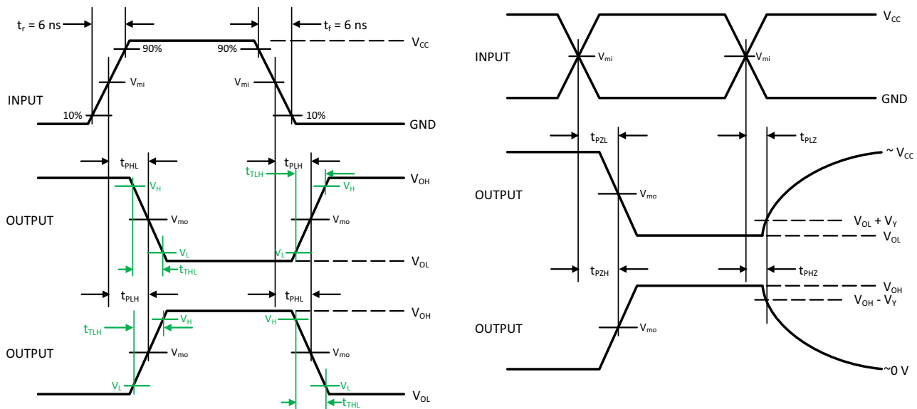
Figure 4. Switching Waveforms
