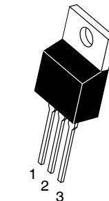
TO-220 CASE 221A STYLE 5
