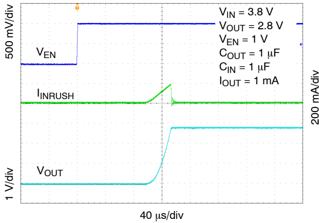
Figure 26. Enable Turn-on Response, C_{OUT} = 1\text{ }\mu\text{F} , I_{OUT} = 1\text{ mA}
