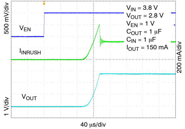
Figure 27. Enable Turn-on Response, C_{OUT} = 1\text{ }\mu\text{F} , I_{OUT} = 150\text{ mA}
