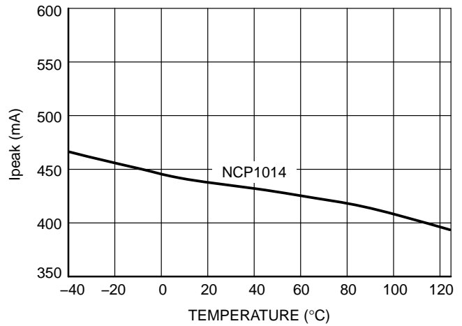
Figure 10. I_{peak-RR} , V_{CC} = 8.0\text{ V} , FB = 3.5\text{ V} vs. Temperature
