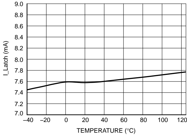
Figure 9. I_{Latch} , FB = 1.5\text{ V} vs. Temperature
