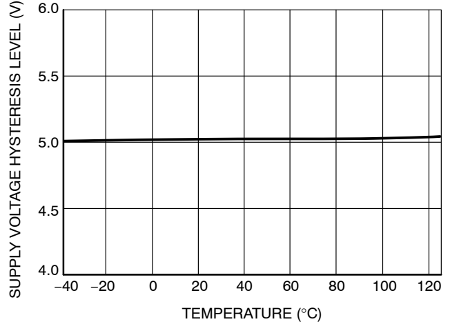
Figure 6. Supply Voltage Hysteresis vs. Junction Temperature (D Version)
