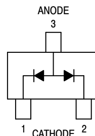
SC-70 (SOT-323) CASE 419 STYLE 4
