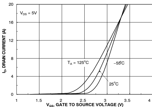
Figure 16. Transfer Characteristics
