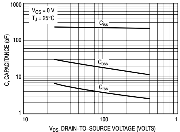
Figure 7b. High Voltage Capacitance Variation
