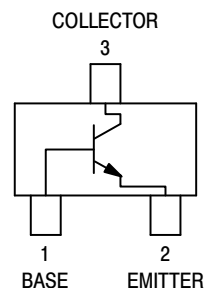
SC-59 CASE 318D STYLE 1
