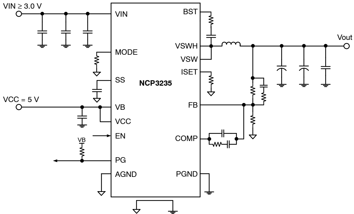
Figure 3. NCP3235 Typical Application Circuit With V_{CC} = 5\text{ V}
