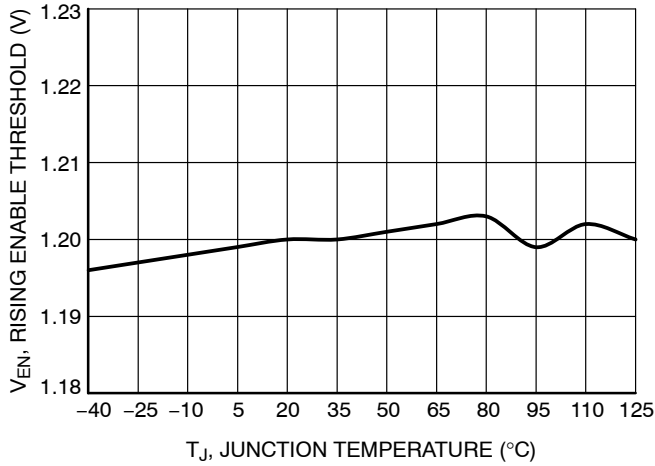
Figure 6. Rising Enable Threshold vs. Temperature
