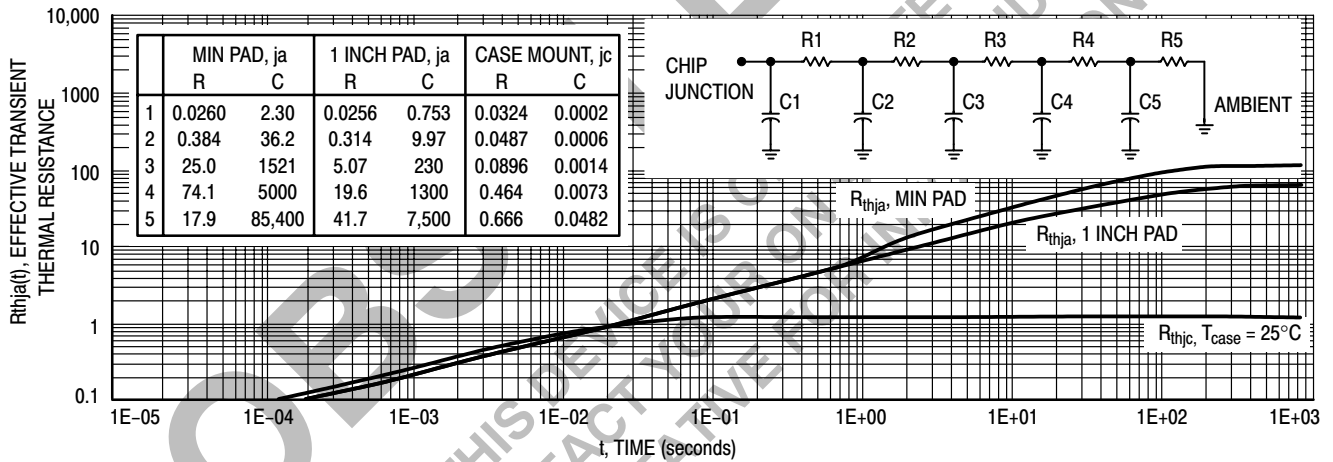
Figure 15. Thermal Response – Various Mounting/Masurement Conditions
