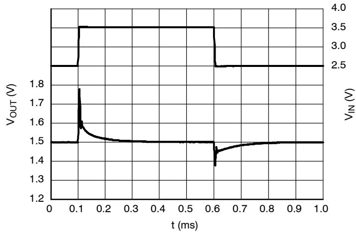
Figure 23. Line Transients, 1.5 V Version, t_{\text{R}} = t_{\text{F}} = 5 \mu\text{s} , I_{\text{OUT}} = 30 \text{ mA}
