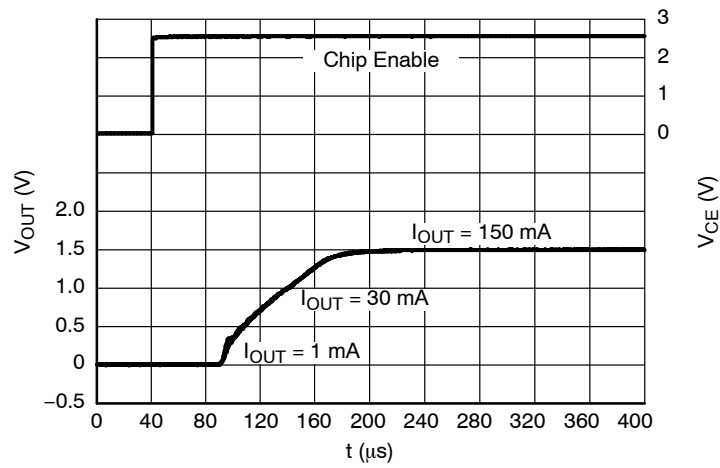
Figure 35. Start-up, 1.5 V Version NCP4681x, V_{IN} = 2.5 V
