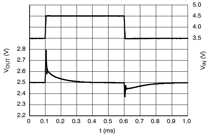
Figure 24. Line Transients, 2.5 V Version, t_{\text{R}} = t_{\text{F}} = 5 \mu\text{s} , I_{\text{OUT}} = 30 \text{ mA}
