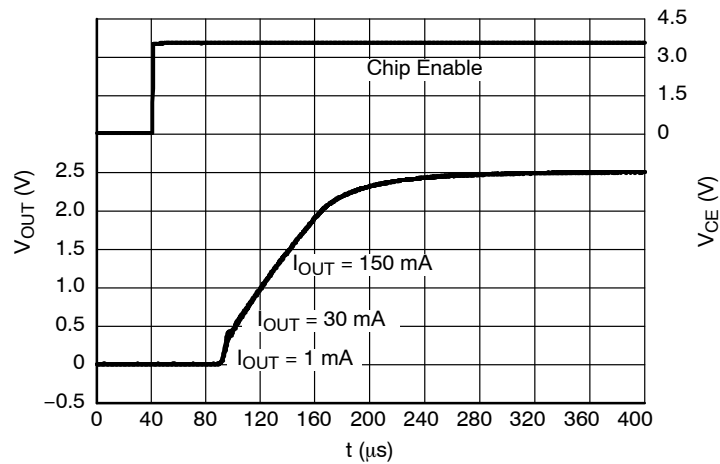
Figure 36. Start-up, 2.5 V Version NCP4681x, V_{IN} = 3.5 V
