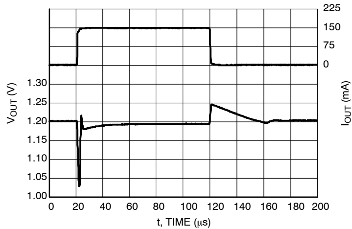
Figure 61. Load Transients, 1.2 V Version, I_{OUT} = 1 - 150 mA, t_R = t_F = 0.5 \mu s, V_{IN} = 2.2 V, AE = 0 V
