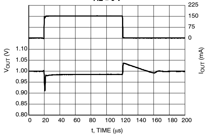
Figure 60. Load Transients, 1.0 V Version, I_{OUT} = 1 - 150 mA, t_R = t_F = 0.5 \mu s, V_{IN} = 2.0 V, AE = V_{IN} V
