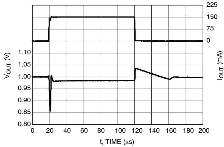
Figure 59. Load Transients, 1.0 V Version, I_{OUT} = 1 - 150 mA, t_R = t_F = 0.5 \mu s, V_{IN} = 2.0 V, AE = 0 V
