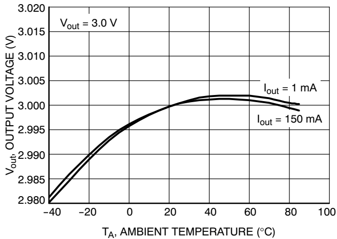
Figure 7. Output Voltage vs. Temperature ( V_{out} = 3.0\text{ V} )
