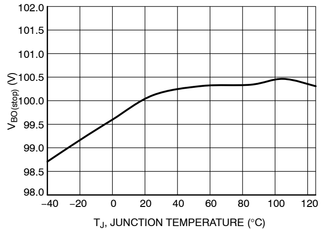
Figure 39. V BO(stop) vs. Temperature
