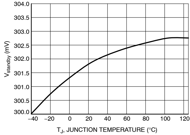
Figure 68. V standby vs. Temperature
