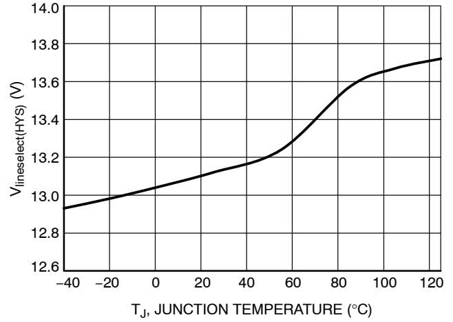
Figure 43. V lineselect(HYS) vs. Temperature
