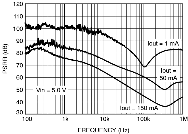
Figure 23. PSRR vs. Frequency NCP4688xx40
