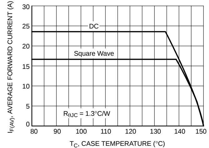
Figure 6. Current Derating
