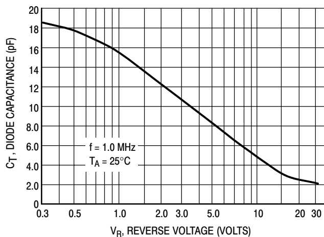
Figure 1. Diode Capacitance
