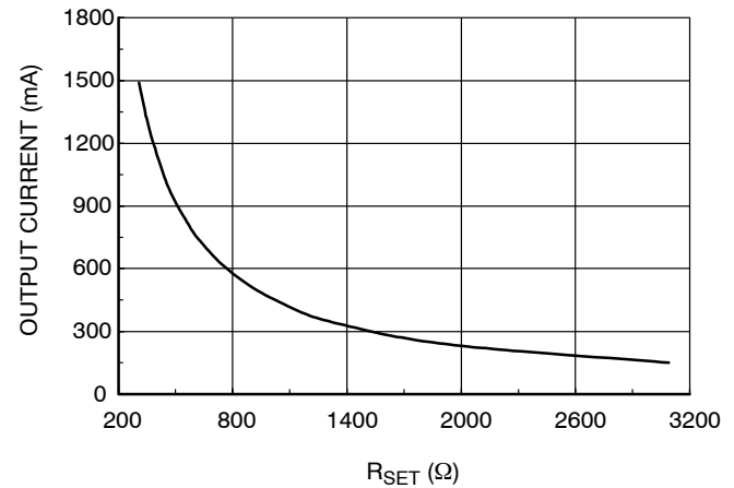
Figure 13. Current Limit vs. Resistor
