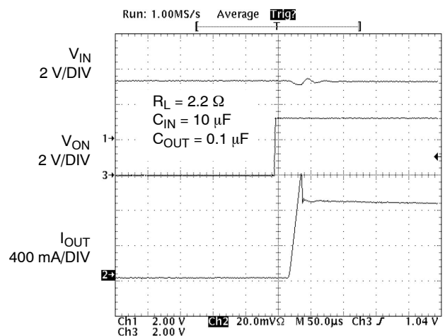
Figure 27. Current Limit Response (Output Shorted to GND by 2.2 \Omega , Moderate Short)
