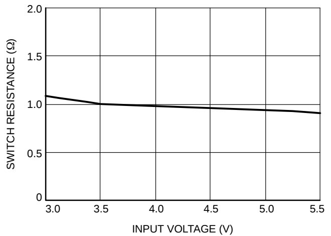
Figure 7. Switch ON Resistance vs. Input Voltage
