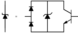
Figure 1. Pin Schematic
