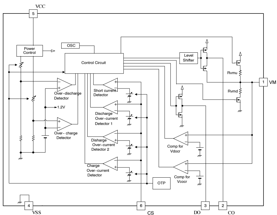
Figure 3. Block Diagram
