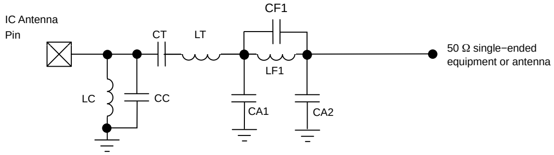
Figure 11. Structure of the Single-ended Antenna Interface for TX Operation to 50 \Omega Single-ended Equipment or Antenna
