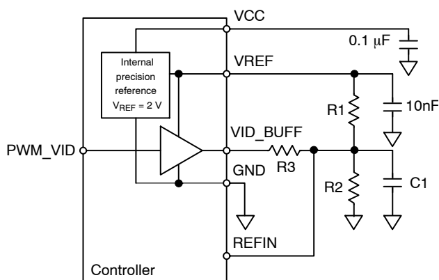
Figure 6. PWM_VID Interface
