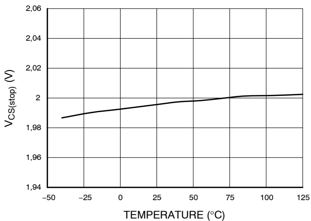
Figure 13. V CS(stop) vs. Temperature
